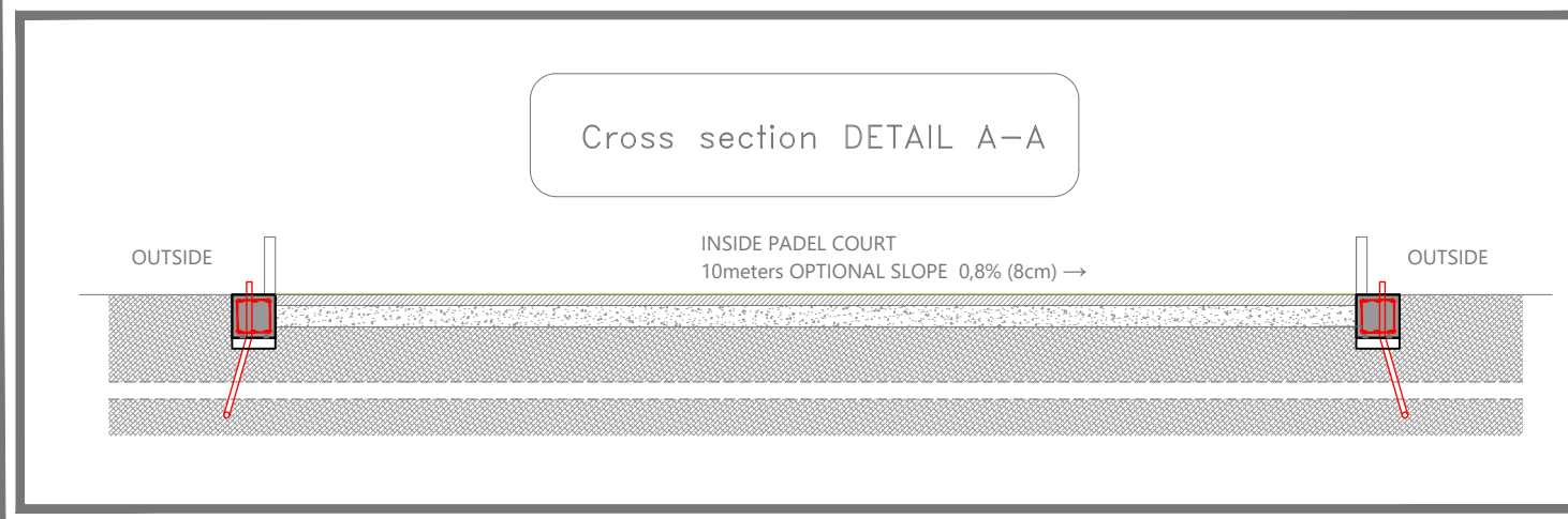
E: 1/75 PERMEABLE BASE FOR STANDARD PADEL COURT
